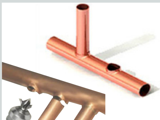
Figure 7.9 Copper Formed Tees – Silver Brazed
