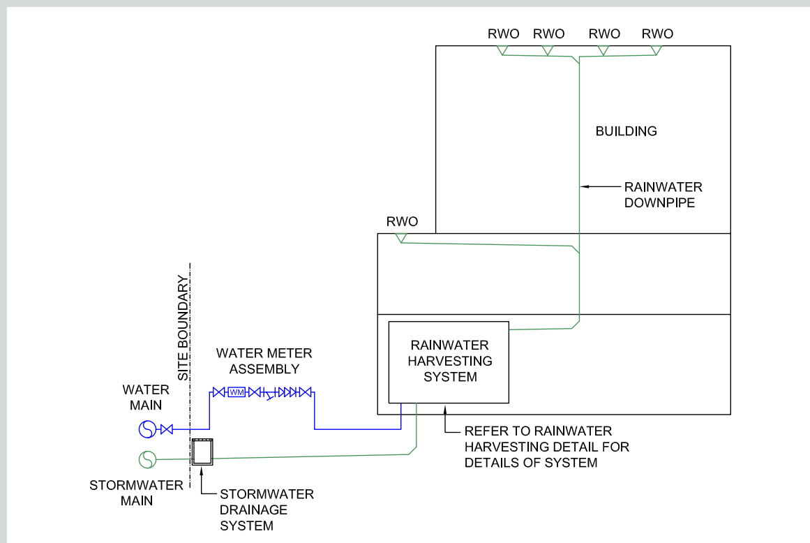
Figure 5.5 Rainwater Building – Concept Design Diagram
