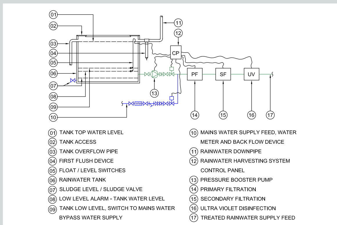
Figure 5.6 Rainwater Harvesting System – Concept Design Diagram
