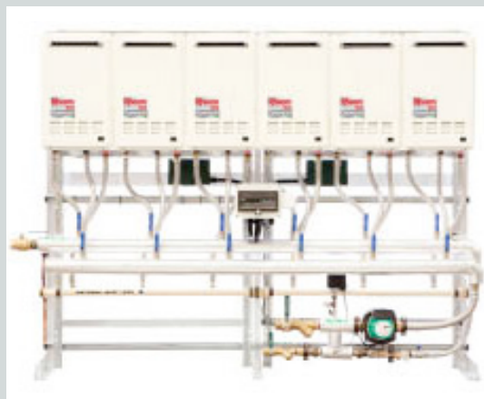
Figure 14.5 Gas continuous flow – commercial
