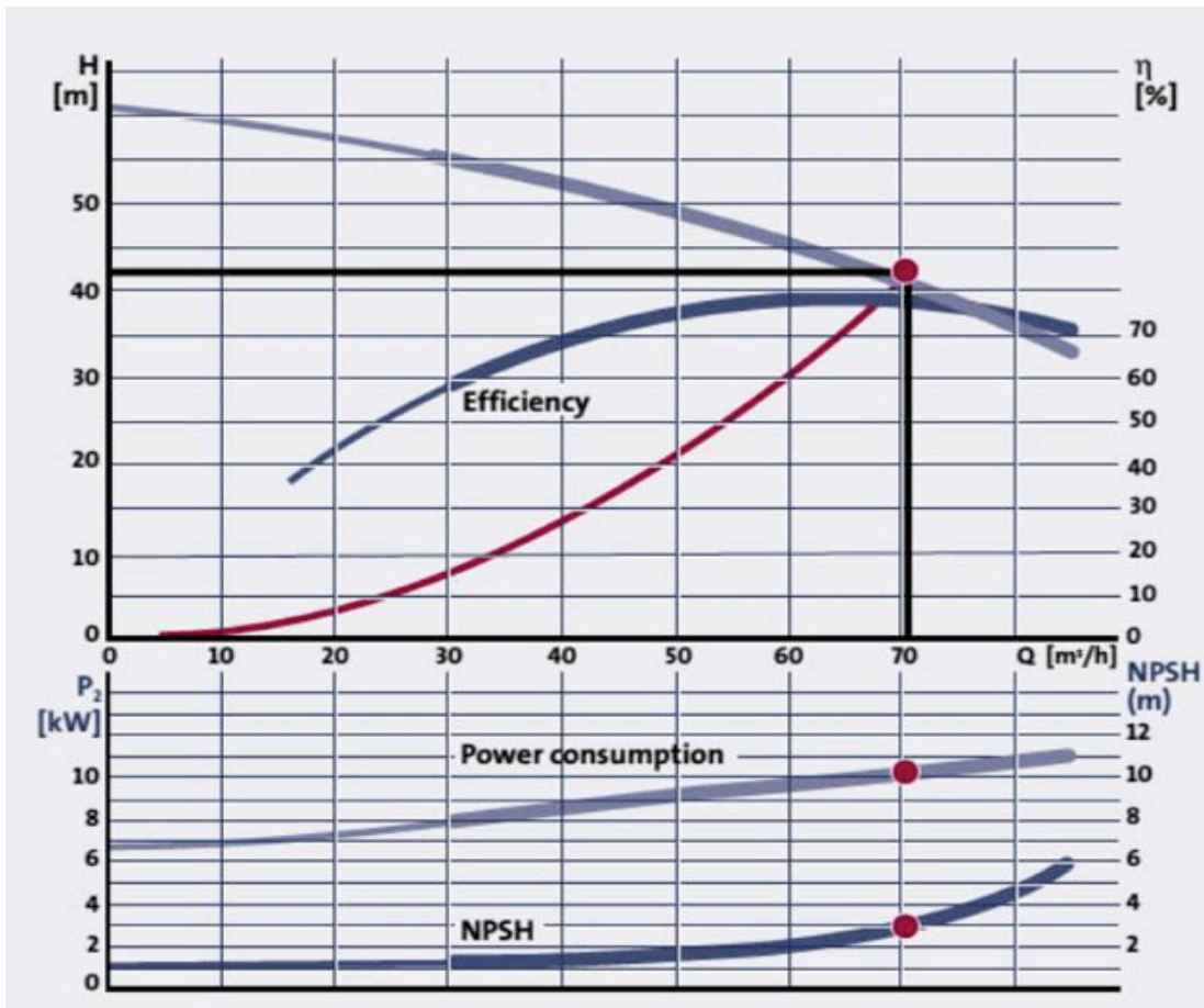
Figure 16.7 Typical Performance Curve for a Centrifugal Pump Head, Power Consumption, Efficiency and NPSH
