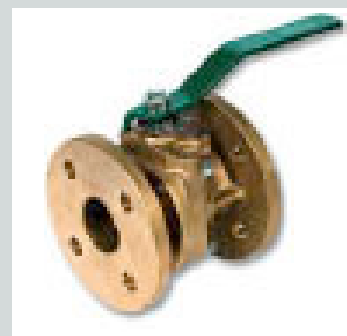
Figure 10.6 Flanged End Connection
