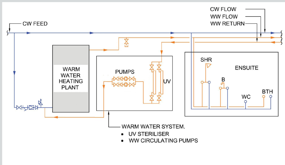
Figure 15.4 Centralised Warm Water System Incorporating a UV System
